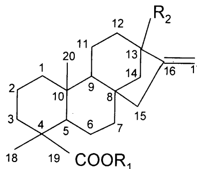
Fig. 1. Molecular Structure of Stevioside
